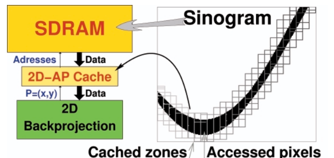
Figure 1. Concept du cache 2D-AP.
