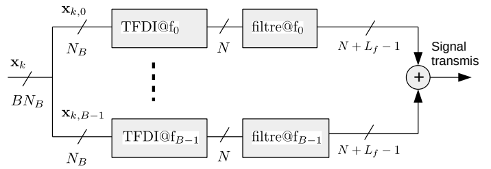
FIGURE 1 – Emission UFMC
