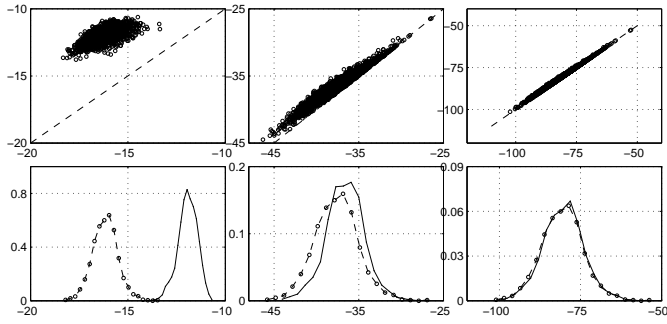
Figure 2: Structure functions versus extrema. Two sides of Relation (12): Scatter plots (top row) and empirical PDFs (bottom row), for j = 5 with (left to right) q = 2, 7 (\simeq q_*^+), 20 .
