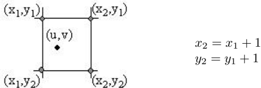
FIG. 1: Interpolating neighborhood
