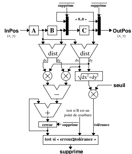
Figure 15: Architecture de l'approximation polygonale
