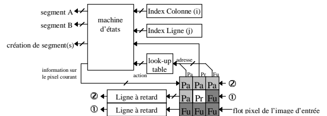
Figure 6: Architecture de l'extraction des segments
